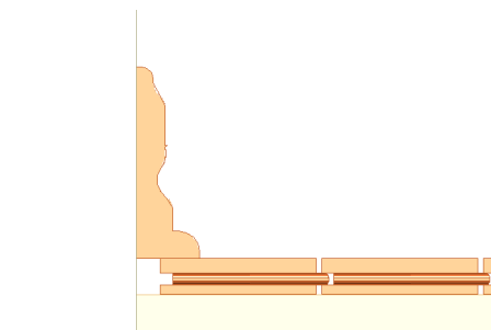
Fig. 11b Baseboard and 1/4-round - section
