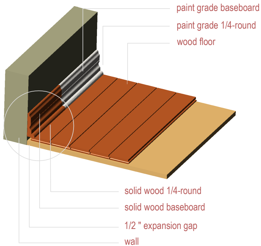
Fig. 11a Baseboard and 1/4-round
