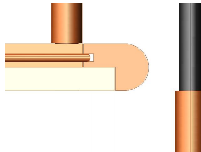
Fig. 12b Nosing - section
